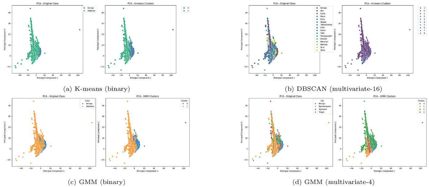
Fig. 3. Principal Components' comparison (original class vs. obtained clusters) for K-means, DBSCAN, and GMM models.
