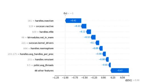
(b) Waterfall plot for the 30405 th instance (anomaly/malicious)
